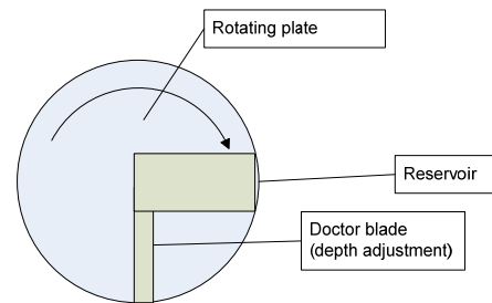
Rotary fluxer top view
