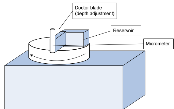
Rotary Fluxer side view
